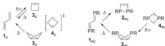
Scheme 1. Known valence isomerizations of singlet C_4H_6 (left) and of P_2C_2R_4 derivatives (right).
