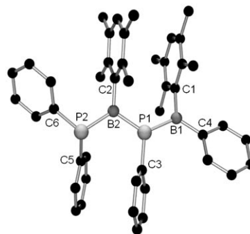
Figure 3. Molecular structure of 8 BP c in the solid state (hydrogen atoms are omitted for clarity). Selected bond lengths [Å] and angles [°]: P1–B1 1.863(7), P1–B2 1.866(7), P2–B2 1.911(8); B1–P1–B2 124.5(3), B1–P1–C3 118.6(3), B2–P1–C3 116.8(3), B2–P2–C5 106.7(3), B2–P2–C6 105.8(3), C5–P2–C6 104.5(3), P1–B1–C4 124.2(5), P1–B1–C1 115.7(5), C4–B1–C1 120.0(6), P1–B2–P2 116.1(4), P1–B2–C2 120.3(5), P2–B2–C2 122.2(5).
