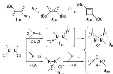
Scheme 2. Photochemical isomerizations of butadiene 1 Ca (top), and two possible mechanisms for the formation of bicyclo[1.1.0]butanes 3 BP and/or butane-1,3-diyls 4 BP (bottom).
