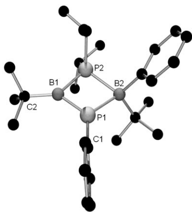
Figure 2. Molecular structure of 5 BP b in the solid state (hydrogen atoms omitted for clarity). Selected bond lengths [Å] and angles [°]: P1–B1 1.795(8), P1–B2 2.014(7), P2–B1 1.949(8), P2–B2 2.053(7); B1–P1–B2 99.8(3), B1–P1–C1 128.4(3), B2–P1–C1 131.8(3), P1–B1–P2 87.2(4), P1–B1–C2 136.1(5), P2–B1–C2 136.7(5), B1–P2–B2 93.6(3), P1–B2–P2 87.2(4).
