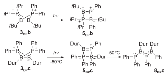
Scheme 5. Photochemical isomerizations of bicyclo[1.1.0]butanes 3 BP b and 3 BP c .
