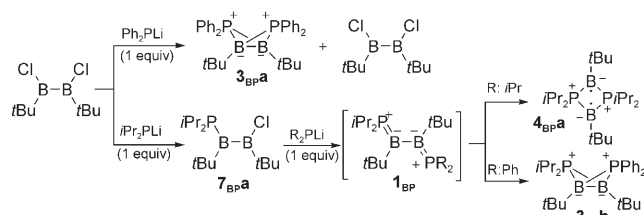
Scheme 3. Synthesis of bicyclo[1.1.0]butane 3 BP a , and syntheses of butane-1,3-diyl 4 BP a and bicyclo[1.1.0]butane 3 BP b via transient butadienes of type 1 BP .
